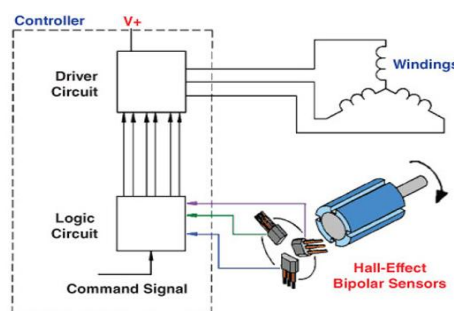
Fig.2 BLDC motor with Hall sensor
