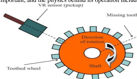
Fig.3 BLDC motor with VR Speed sensor
