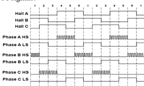
Fig.5 PWM commutation scheme
