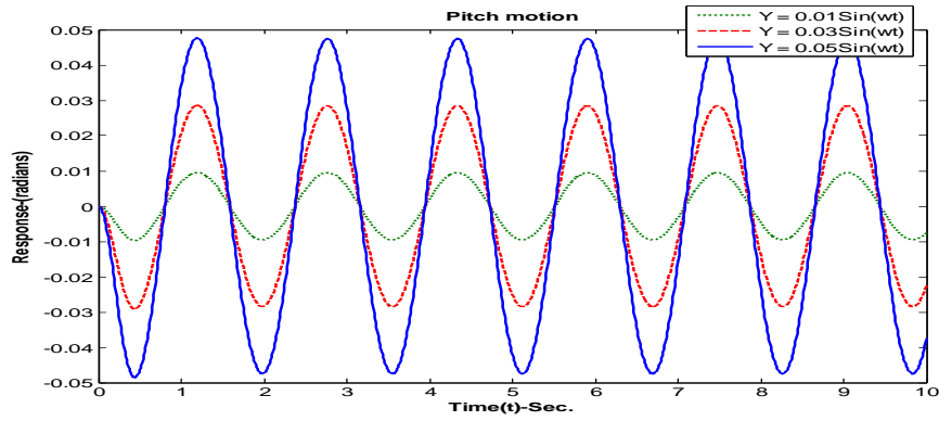
Fig.3 Pitch motion response of the vehicle at v=11.5\text{km/hr}
