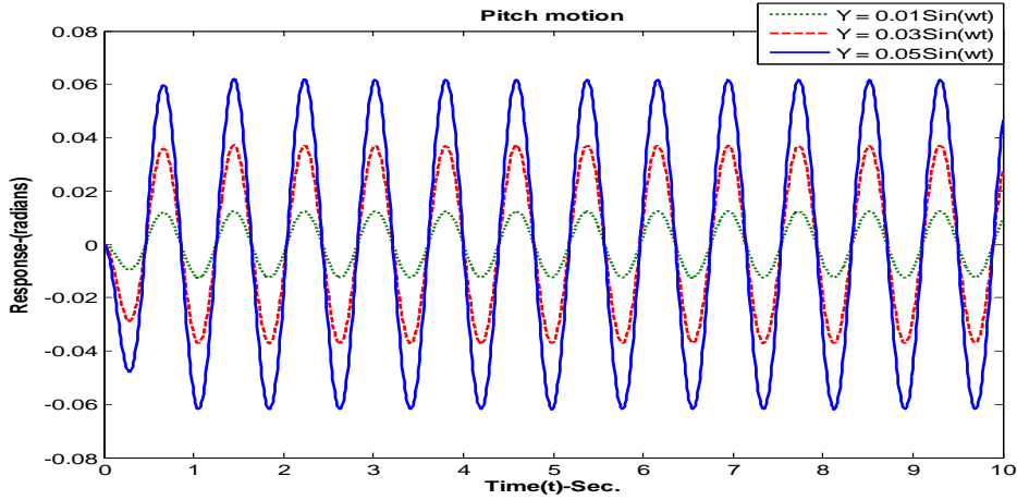
Fig.7 Pitch motion response of the vehicle at v=22.9 km/hr
