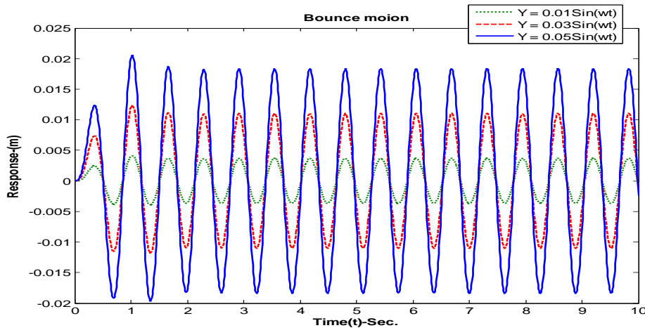
Fig.8 Bounce motion response of the vehicle at v=28.65 km/hr
