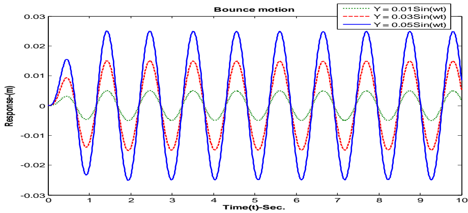
Fig.5 Pitch motion response of the vehicle at v=17.2 \text{ km/h}
