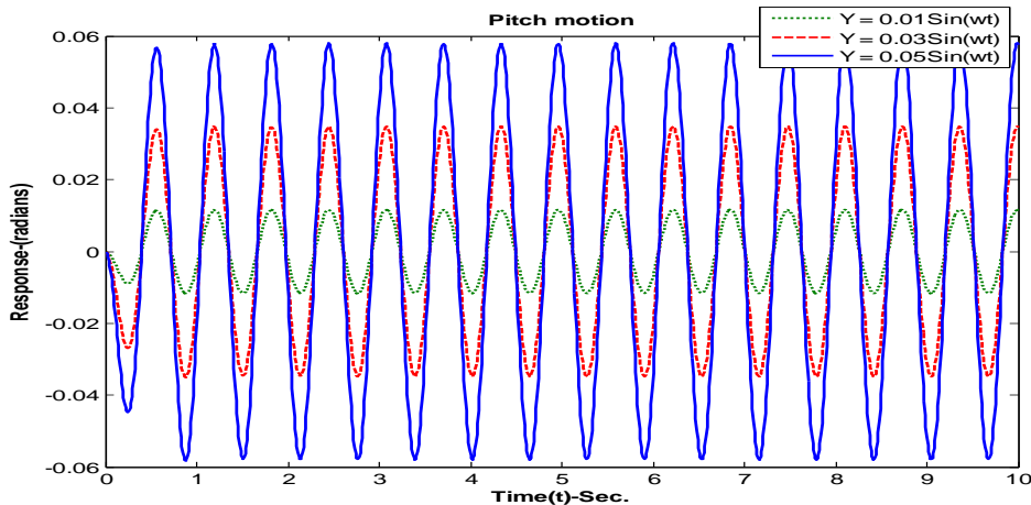
Fig.9 Pitch motion response of the vehicle at v=28.65 km/hr
