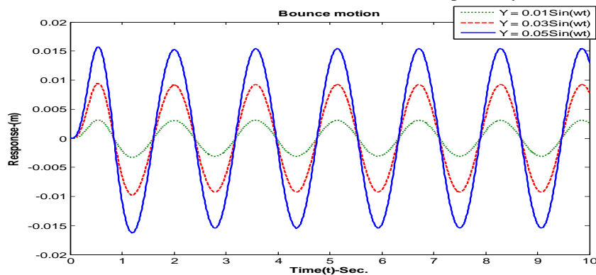
Fig.2 Bounce motion response of the vehicle at v=11.5km/h
