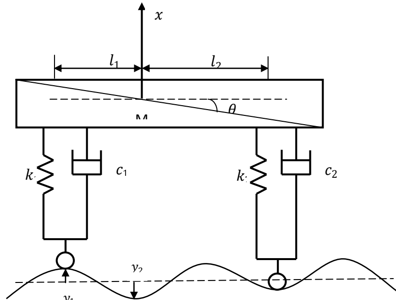
Figure 1: Lagrangian of the two-degree-of-freedom half car model.
