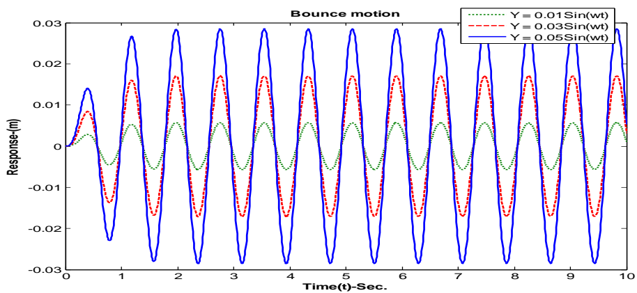
Fig.6 Bounce motion response of the vehicle at v=22.9 \text{ km/hr}
